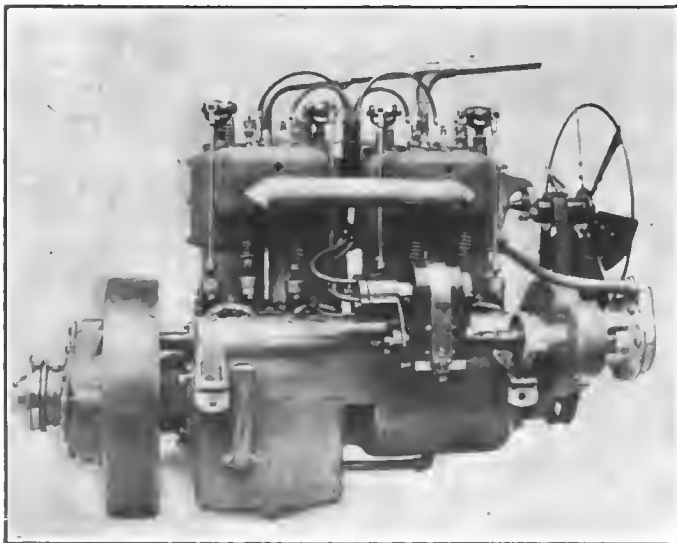
Fig. 3—Showing the right side of Reo motor
